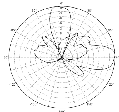
E/H-plane Radiation Pattern 5500 MHz
